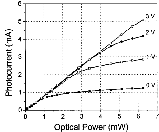
Fig. 2. Optical input power versus photocurrent of the photodetector under various reverse biases.
