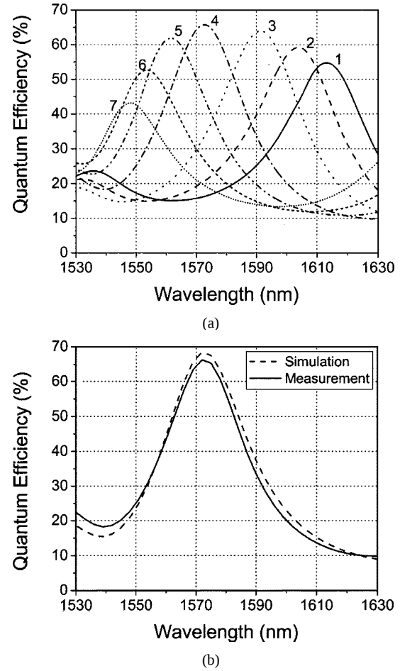
Fig. 1. (a) Spectral quantum efficiency measurements of the fabricated detectors after consecutive recess etches. (b) The theoretical calculation and experimental quantum efficiency measurement of a detector whose resonance had been tuned to 1572 nm.
