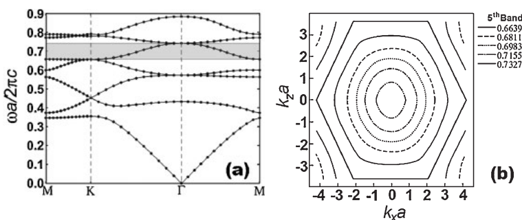
Fig. 5. (a) Calculated TE polarized band structure. Shaded band (fifth band) covers the frequencies where the structure possess negative index of refraction. (b) Equal-frequency contours of the fifth band in the full Brillouin zone. The contours are nearly circular (i.e. isotropic) and shrink with increasing frequency.
