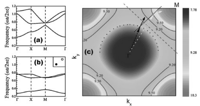
Fig. 8. (a) Calculated TM-polarized bands for the metallic photonic crystal, and (b) the metaldielectric crystal. (c) Equal-frequency contours (solid curves) are shown for the metaldielectric PC. Dotted circle is the free-space equal-frequency contour at 9.5 GHz. Free-space wave vector (black dashed arrow), free-space group velocity (black solid arrow), wave vector of the refracted waves in the PC (white dashed arrow), group velocity inside the PC (white solid arrow) are drawn.
