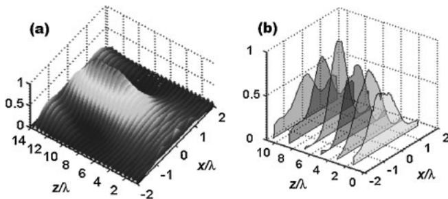
Fig. 7. (a) Simulated 2D intensity profile in the image plane. z = 0 corresponds to the PC–air interface. (b) Measured lateral intensity profiles along the propagation direction. Measurements are performed at six different positions z/\lambda = 1.78, 3.56, 5.34, 7.12, 8.90, \text{ and } 10.68 .
