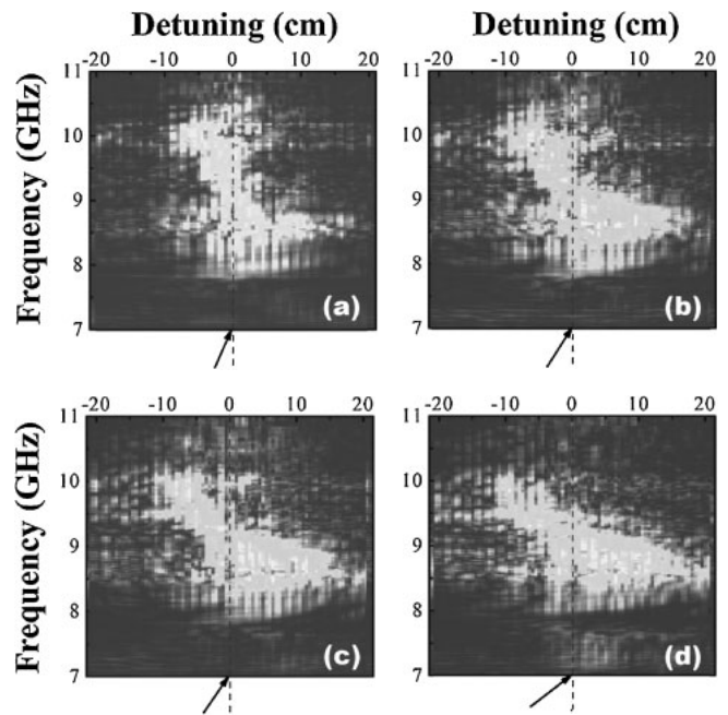
Fig. 9. Measured electric field intensities along the PC-air interface for incident angles of (a) \theta = 15^\circ , (b) \theta = 25^\circ , (c) \theta = 35^\circ , and (d) \theta = 45^\circ . The intensities are plotted as a function of frequency. Upto 9.2 GHz structure positively refracting, between 9.2 and 10.3 GHz structure refracts negatively.
