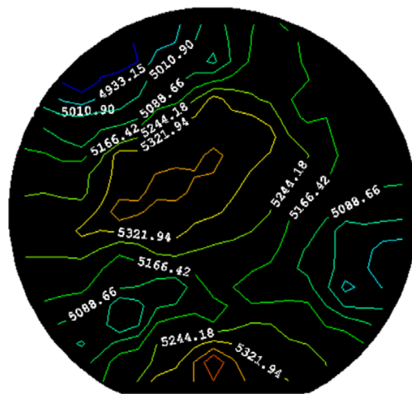
Fig. 6. Sheet resistance map of the 2-inch GaN/AlN/SiN x /Si (111) structure with a nitridation time of 60 s (sample C). The average sheet resistance and resistance uniformity is 5178 \Omega\text{sq}^{-1} and 96.5%, respectively.
