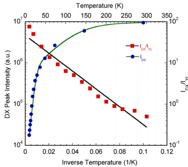
Fig. 11. D^0X_A related PL intensity as a function of an inverse temperature and the temperature dependence of the relative intensities ( I_{DX}/I_{YL} ) for sample D. The solid line is drawn to calculate the activation energies by using Eq. (1). The black solid line represents the exponential fit to the temperature behavior of the I_{DX}/I_{YL} ratio.
