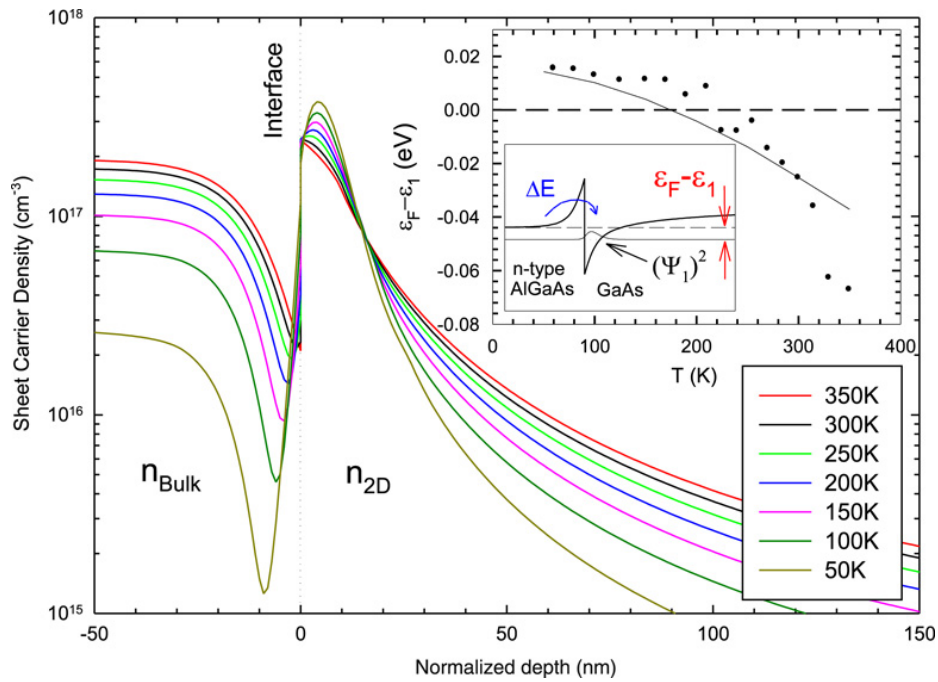
Fig. 4. Temperature dependent simulated carrier densities of n-AlGaAs barrier layer ( n_{Bulk} ) and the 2DEG ( n_{2D} ). Insert: Temperature dependent first subband energy with respect to the Fermi level for results extracted by QMSA results (filled circles) and results calculated with simulations (solid line). Conduction band diagram with Fermi level, effective barrier height ( \Delta E ), first subband energy and the probability density of the 2DEG electron ( (\psi_1)^2 ) is also shown in a box.
