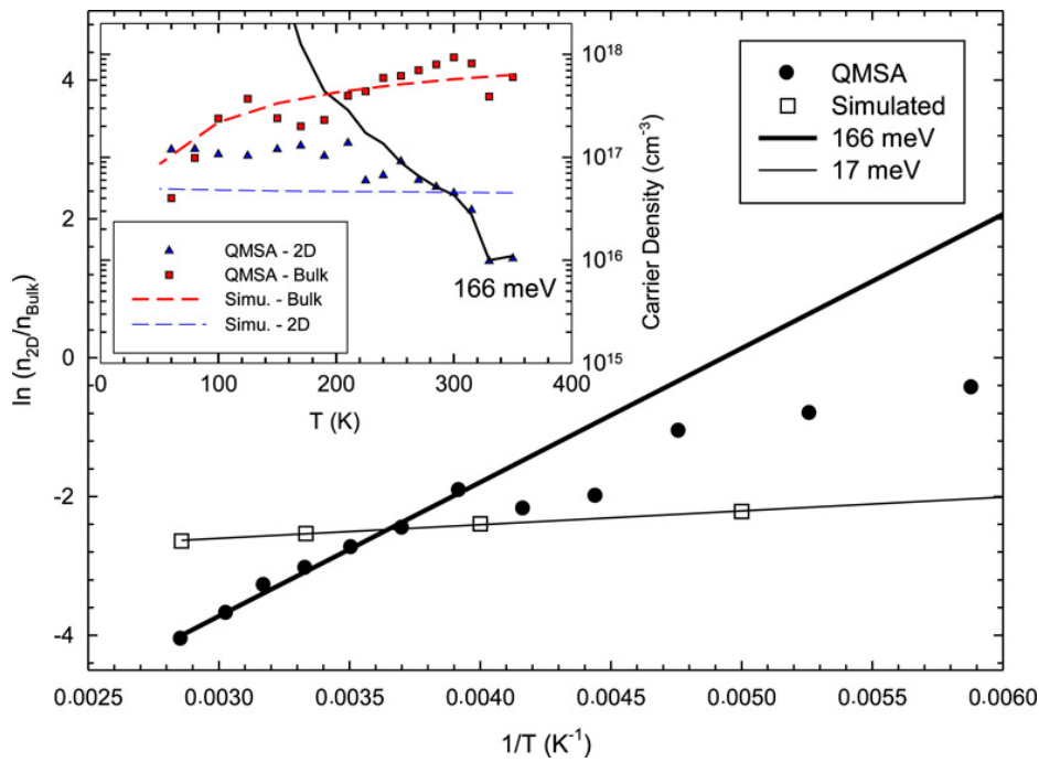
Fig. 5. Logarithm of the n_{2D}/n_{Bulk} as a function of the reciprocal temperature for the results extracted by QMSA and the simulation results. Fitted \Delta E values are shown as full lines. Insert: Temperature dependent carrier densities of 2DEG carrier extracted by QMSA (blue triangles), bulk carrier extracted by QMSA (red squares), simulational 2DEG carrier (blue dashed line) and simulational bulk carrier (red dashed line). Full line shows the n_{2D} calculated with using \Delta E = 166 meV and n_{Bulk} values extracted by QMSA. (For interpretation of the references to colour in this figure legend, the reader is referred to the web version of this article.)
