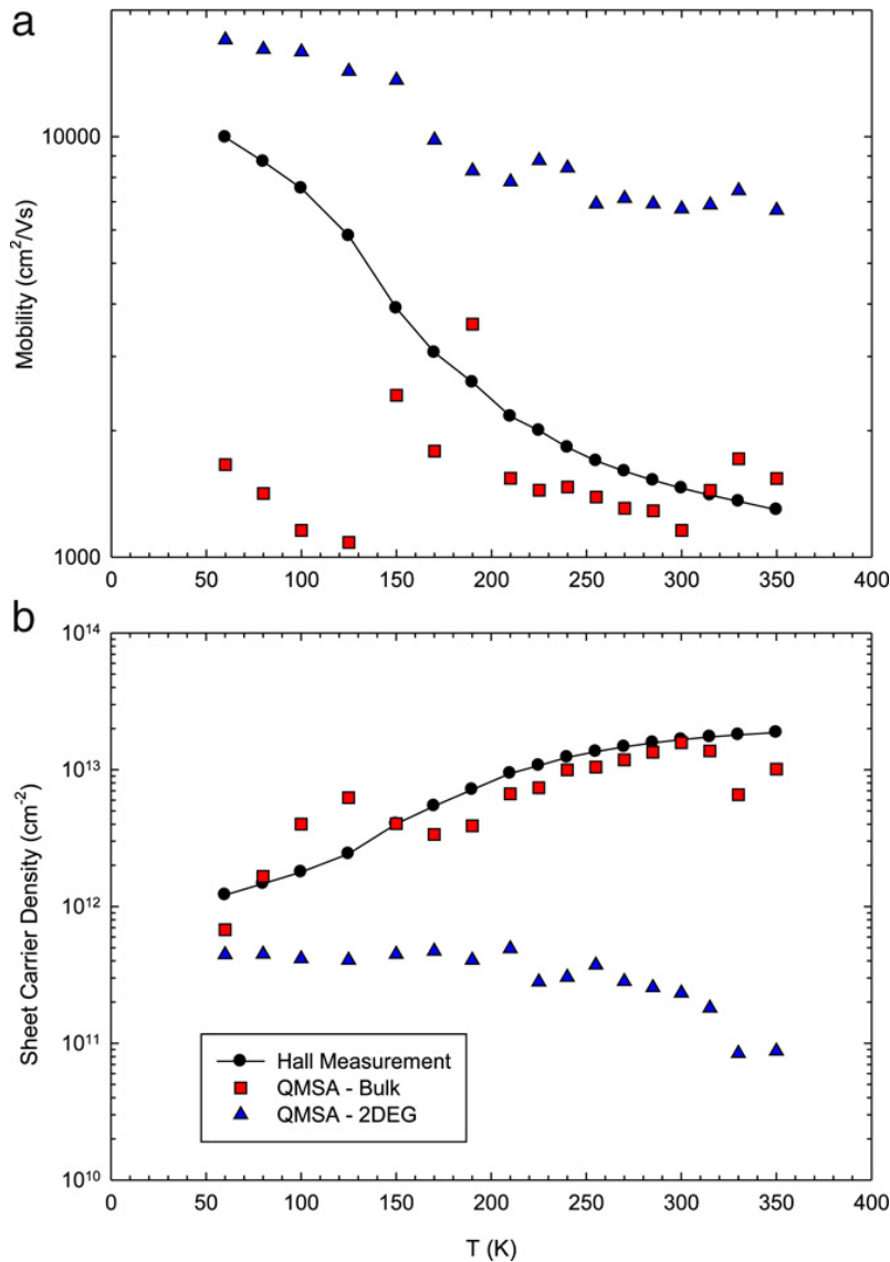
Fig. 2. Temperature dependent mobilities (a) and sheet carrier densities (b) of the carriers extracted by QMSA. Hall results are also shown for comparison.
