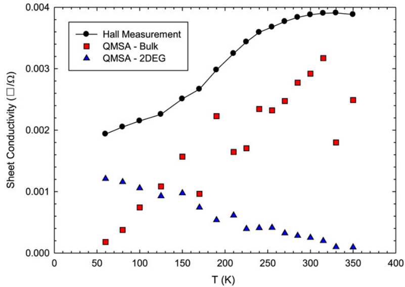
Fig. 3. Temperature dependent sheet conductivities calculated with Hall results and results extracted by QMSA.
