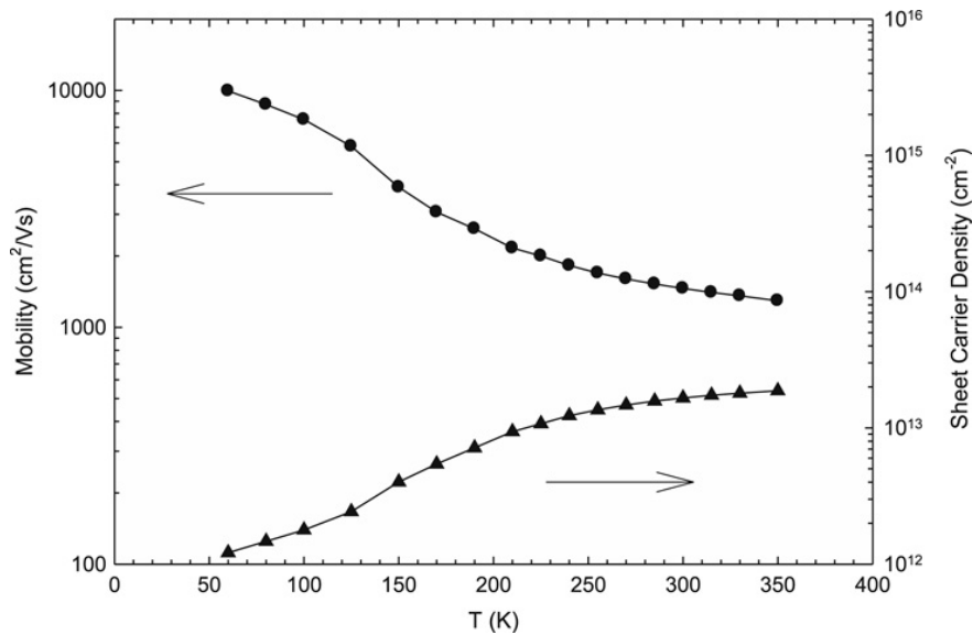
Fig. 1. Temperature dependent Hall mobility and Hall sheet carrier density.
