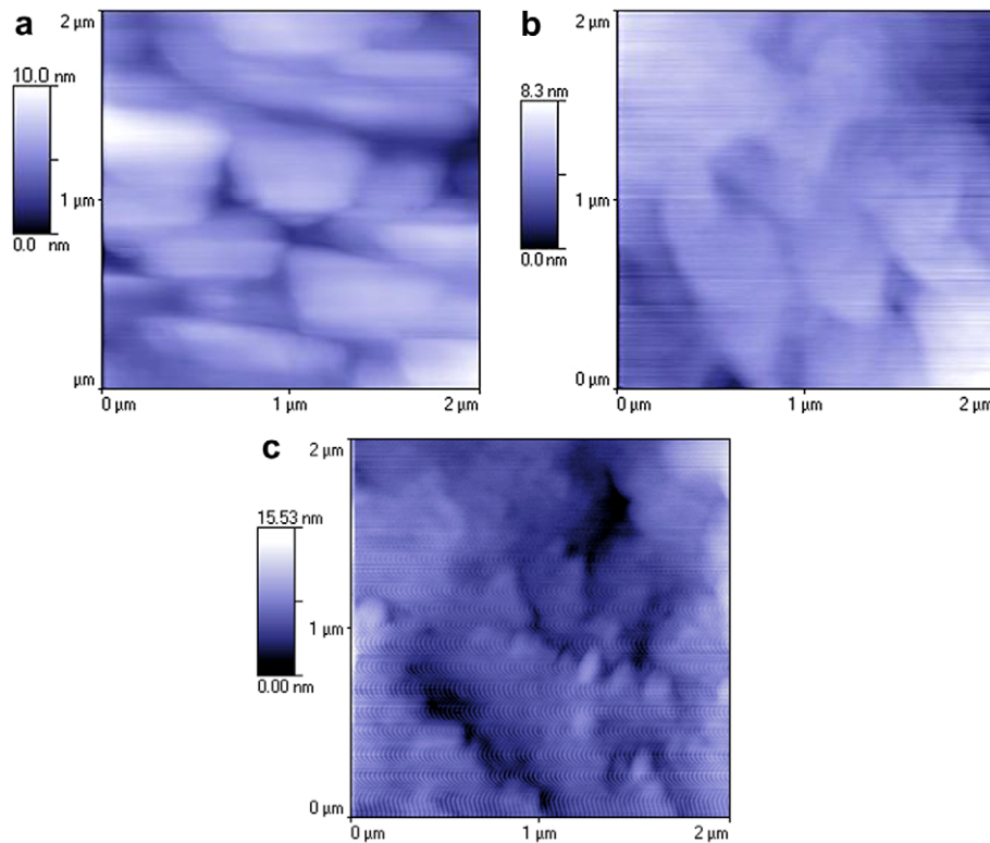
Fig. 3. AFM images of AFM scans (2 μm × 2 μm scans) of GaN films in (a) sample A, (b) sample B, and (c) sample C.
