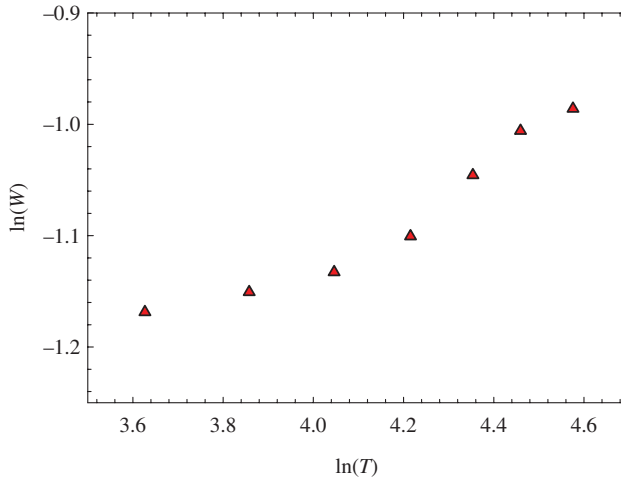
Figure 1. Plot of \ln(W) versus \ln(T) for AlGaIn.
