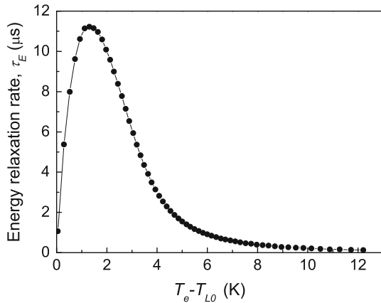
Fig. 11. Energy relaxation time ( t_e ) versus T_e - T_{L0} for the \text{Al}_{0.83}\text{In}_{0.17}\text{N}/\text{AlN}/\text{GaN} heterostructure. The solid curves through the experimental data points are intended as a guide for the eye.
