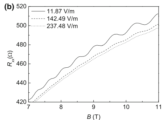
Fig. 2. Experimental results showing the effects of (a) temperature and (b) applied electric field on the magnetoresistance R_{xx}(B) measured for an \text{Al}_{0.83}\text{In}_{0.17}\text{N}/\text{AlN}/\text{GaN} heterostructure sample.
